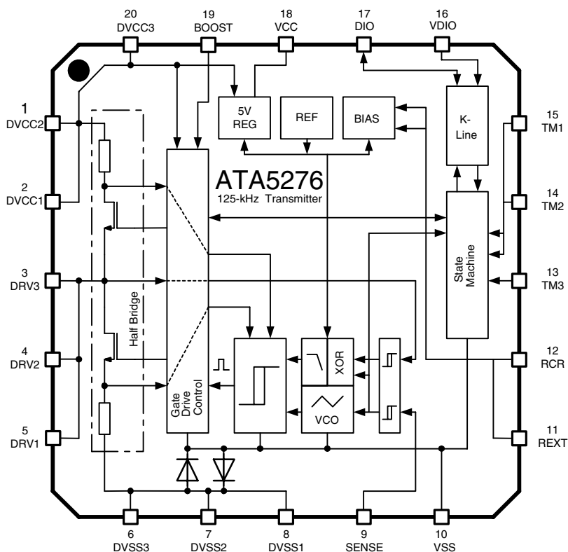
Figure 2-1. Block Diagram
